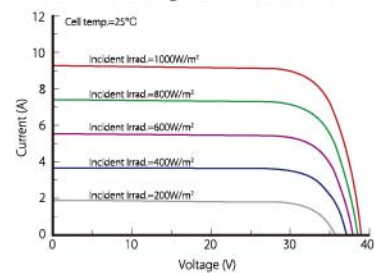
Current-Voltage Curve (LR6-60PB-285M)
